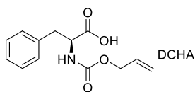
Aloc-Phe-OH·DCHA
