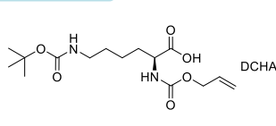
Aloc-Lys(Boc)-OH·DCHA
