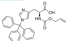
Aloc-His(Trt)-OH
