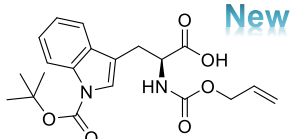
Aloc-Trp(Boc)-OH
