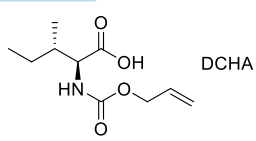
Aloc-Ile-OH·DCHA
