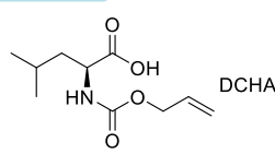
Aloc-Leu-OH·DCHA
