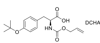
Aloc-Tyr(tBu)-OH·DCHA
