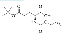
Aloc-Glu(OtBu)-OH
