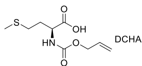
Aloc-Met-OH·DCHA
