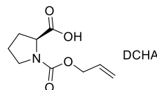
Aloc-Pro-OH·DCHA
