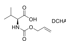
Aloc-Val-OH·DCHA
